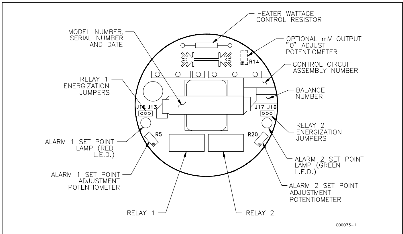
Figure 3-2. Control Circuit Outline Drawing
