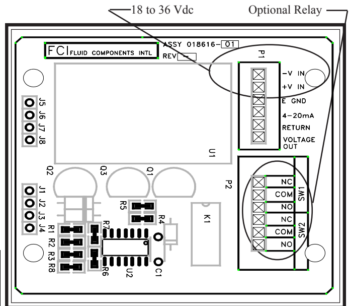
Customer Wiring Diagram
