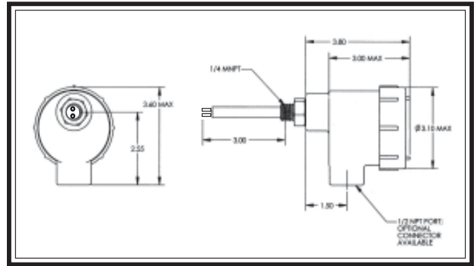
Installation Outline Diagram
